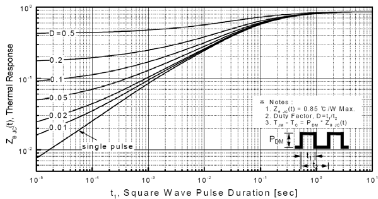
Figure 11-1. Transient Thermal Response Curve for WGP7N60
