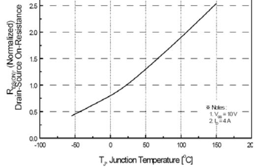
Figure 8. On-Resistance Variation vs Temperature
