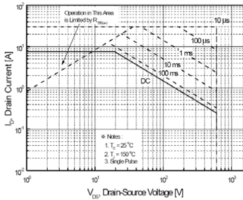
Figure 9-1. Maximum Safe Operating Area for WGP7N60
